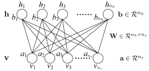
Fig. 1. Structure of an RBM.
