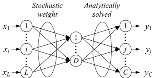
Fig. 2. Single hidden layer RWNN.
