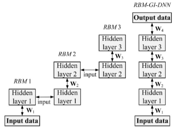
Fig. 4. Training process.
